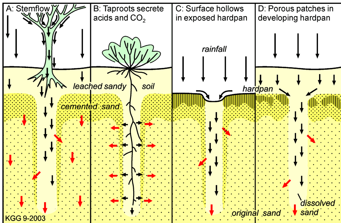
Figure 6: Alternative ways in which the downward flow of water can become focussed to generate solution pipes (see text). Black arrows are aggressive water flow and red arrows are saturated water. Note, the alternatives are not mutually exclusive, they could all contribute in different settings.
